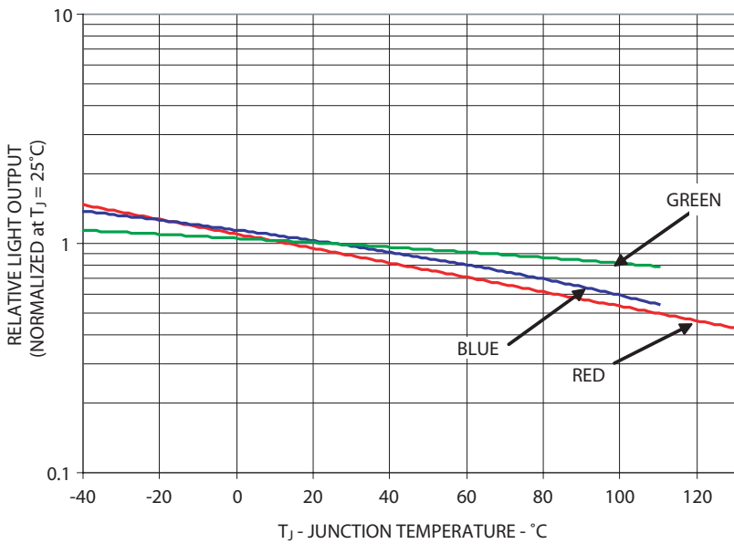
Relative Light Output vs. Junction Temperature
